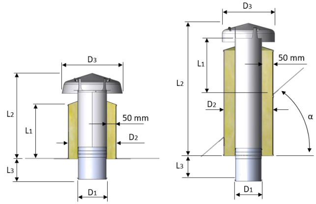
DIMENSION OVERVIEW - INSULATED VARIANTS
